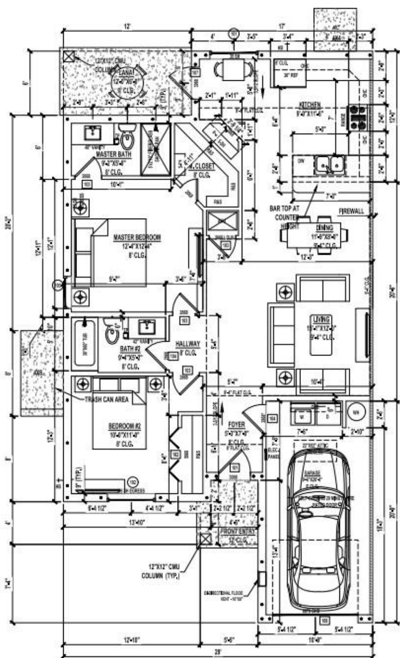
TYPICAL DIMENSION PLAN
