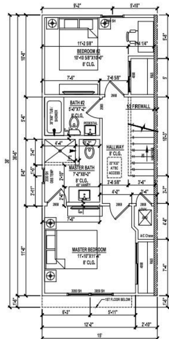
TYPICAL 2ND FLOOR PLAN
