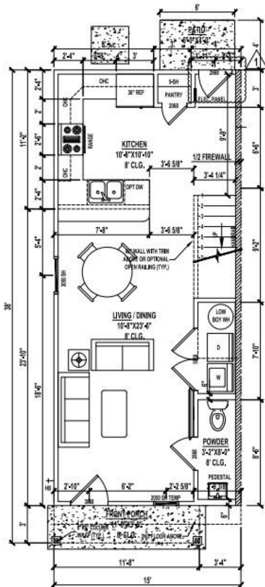
TYPICAL 1ST FLOOR PLAN
