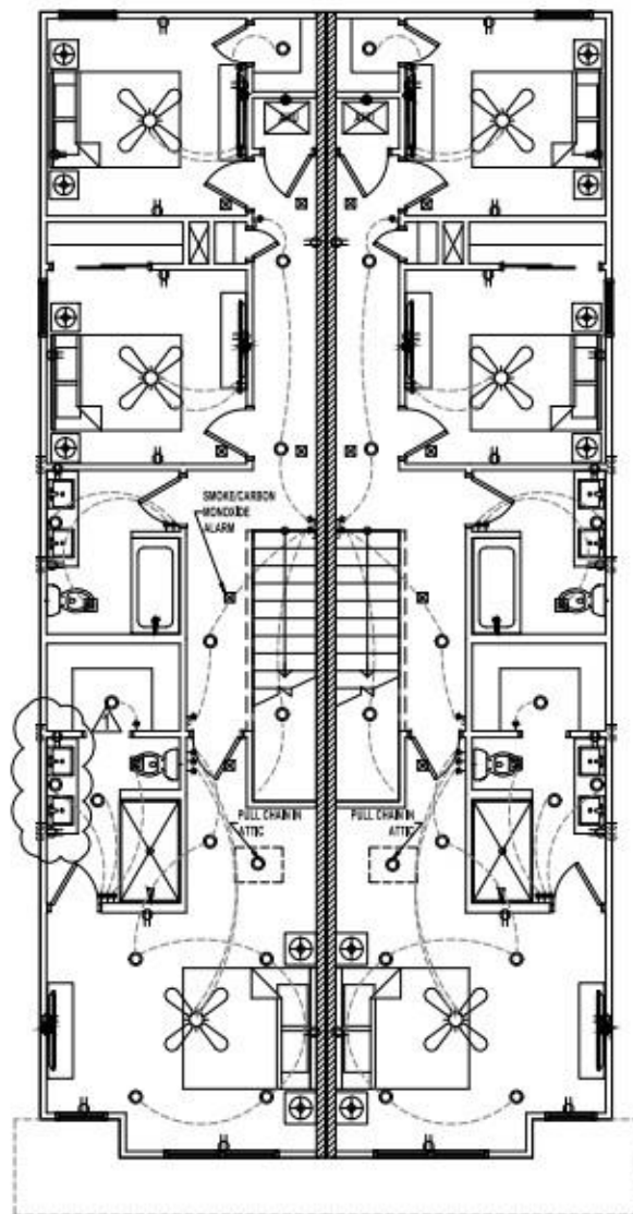
TYPICAL ELECTRIC PLAN A SCALE 1/4" = 1'-0"
