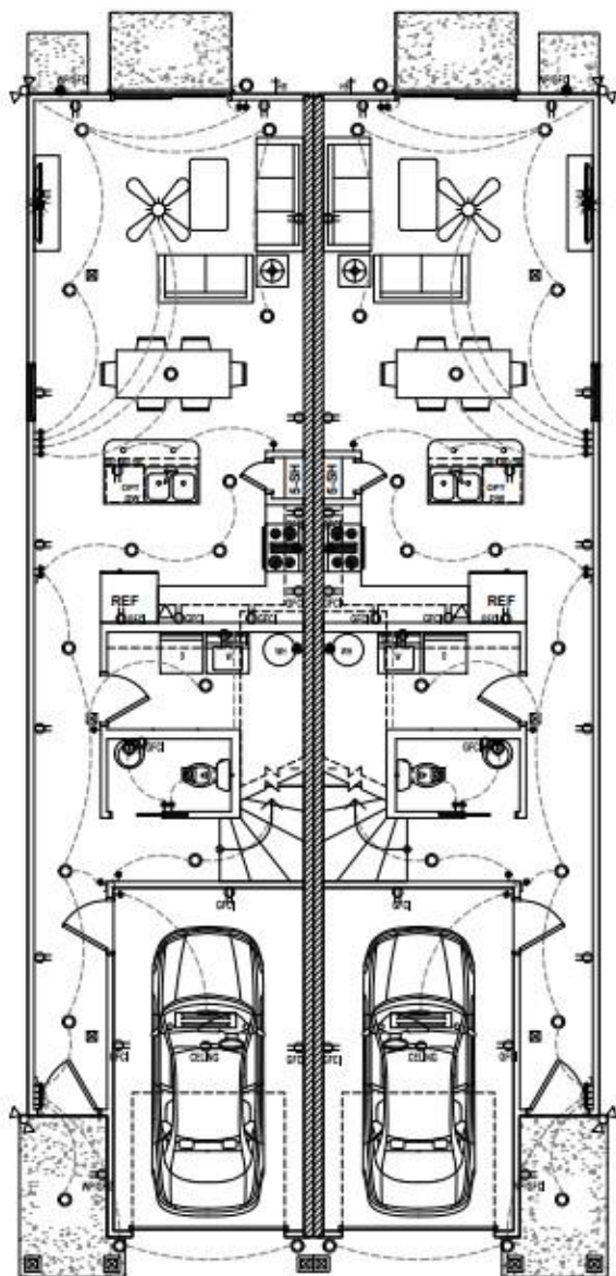
TYPICAL ELECTRIC PLAN A SCALE 1/4" = 1'-0"
