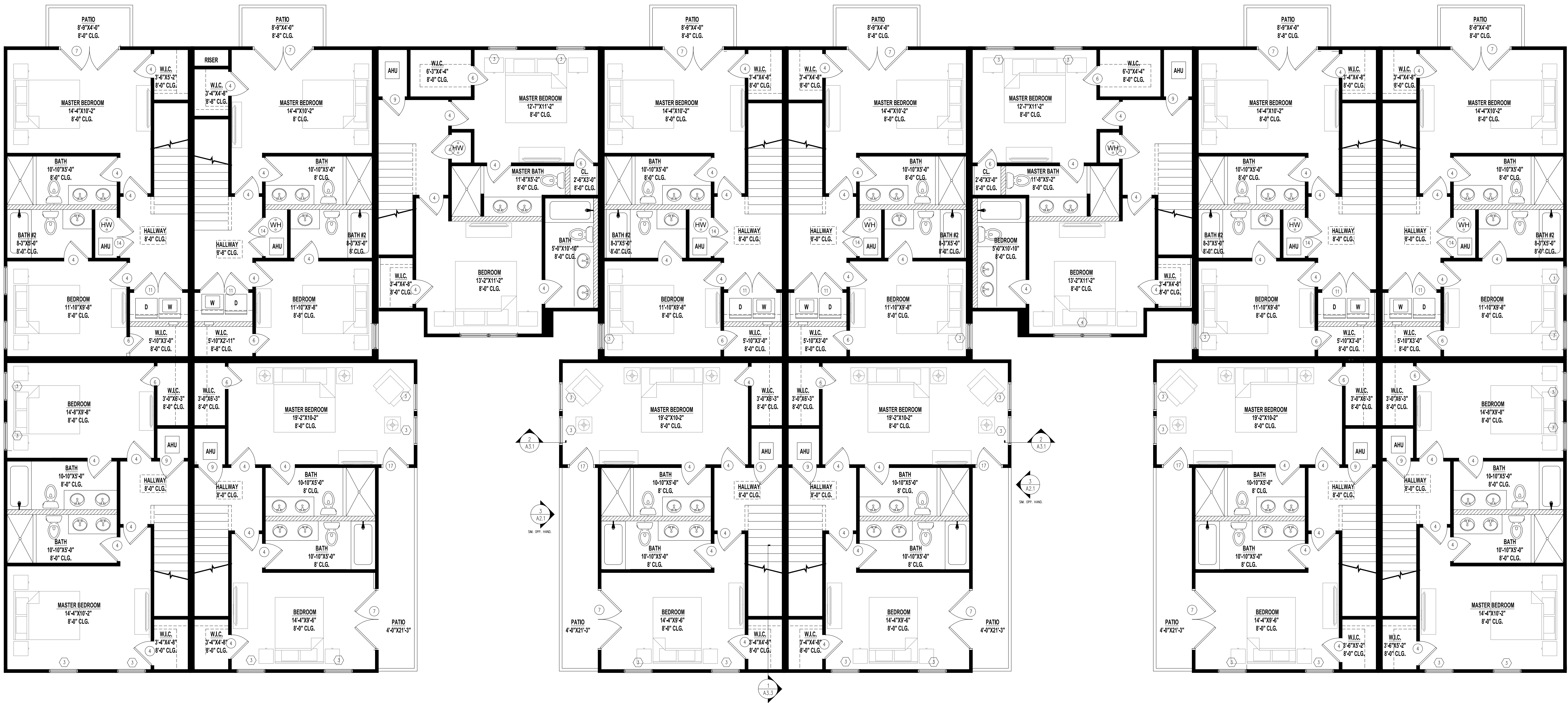
1 2ND FLOOR PLAN: 14-PLEX A1.1 SCALE: 3/16" = 1'-0"
