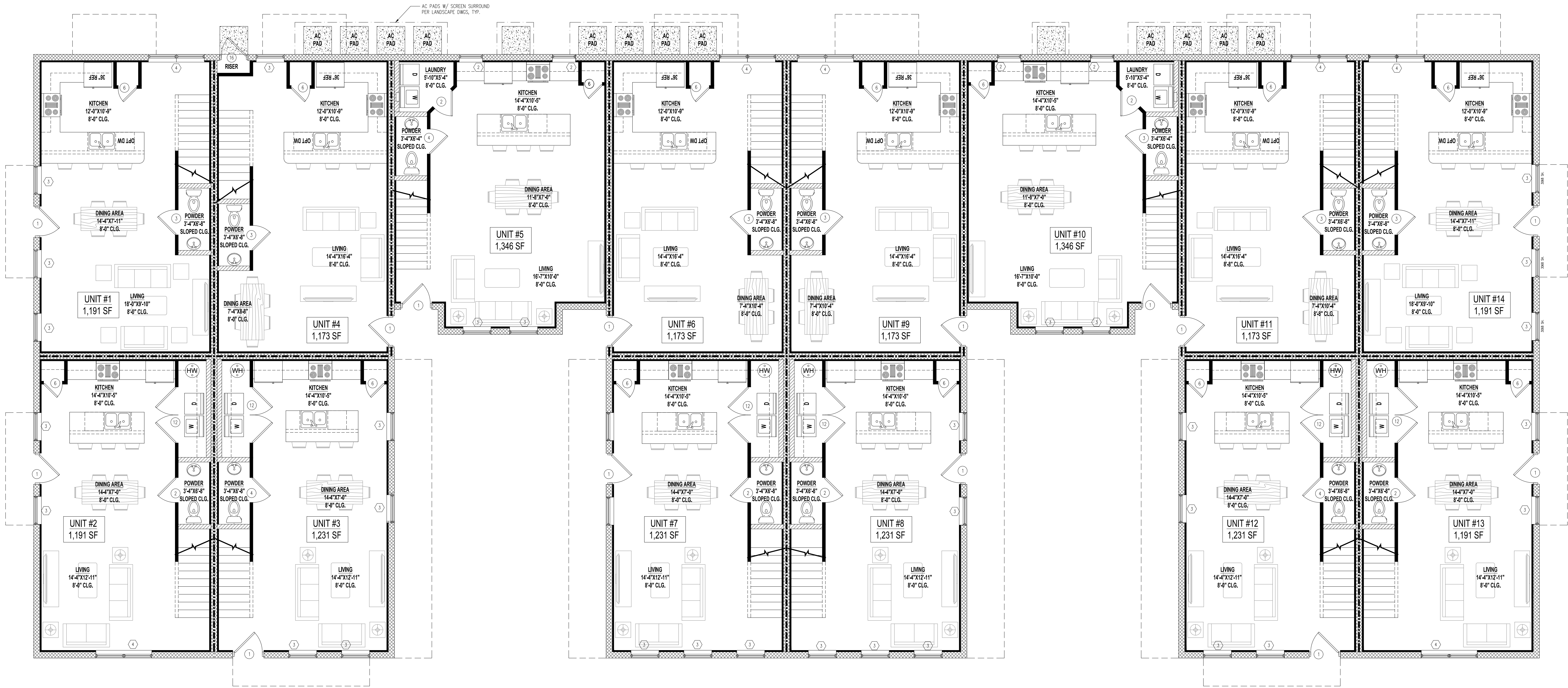
1 1ST FLOOR PLAN: 14-PLEX A1.1 SCALE: 3/16" = 1'-0"
