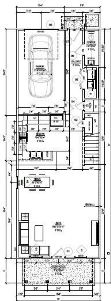
1ST FLOOR PLAN | END UNIT
