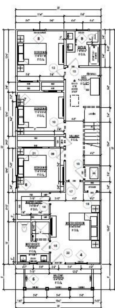
2ND FLOOR PLAN | END UNIT
