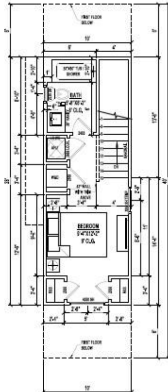
2 2ND FLOOR PLAN SCALE 1/8" = 1'-0"
