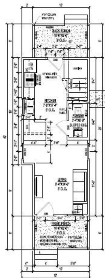
1 1ST FLOOR PLAN SCALE 1/8" = 1'-0"
