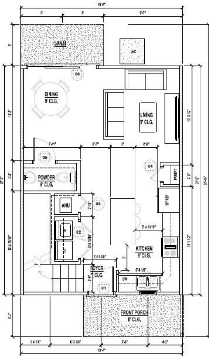
1ST FLOOR PLAN | UNIT C 2BD
