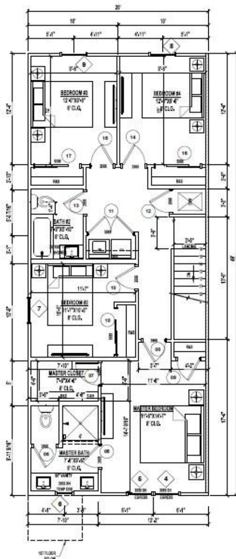
2 2ND FLOOR PLAN END UNIT
